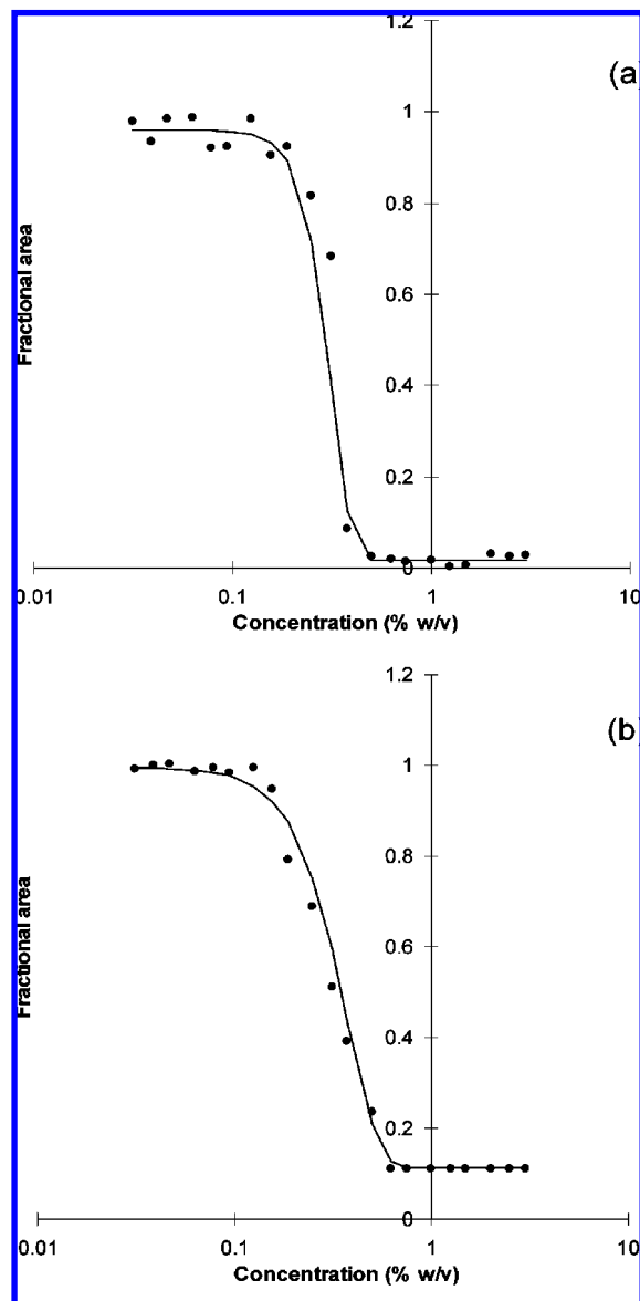
Figure 2. Inhibition profile of Voidomato seeds extract against Listeria monocytogenes with conductance technique (a) and count technique (b): (●) observed fractional area; (—) predicted fractional area.
